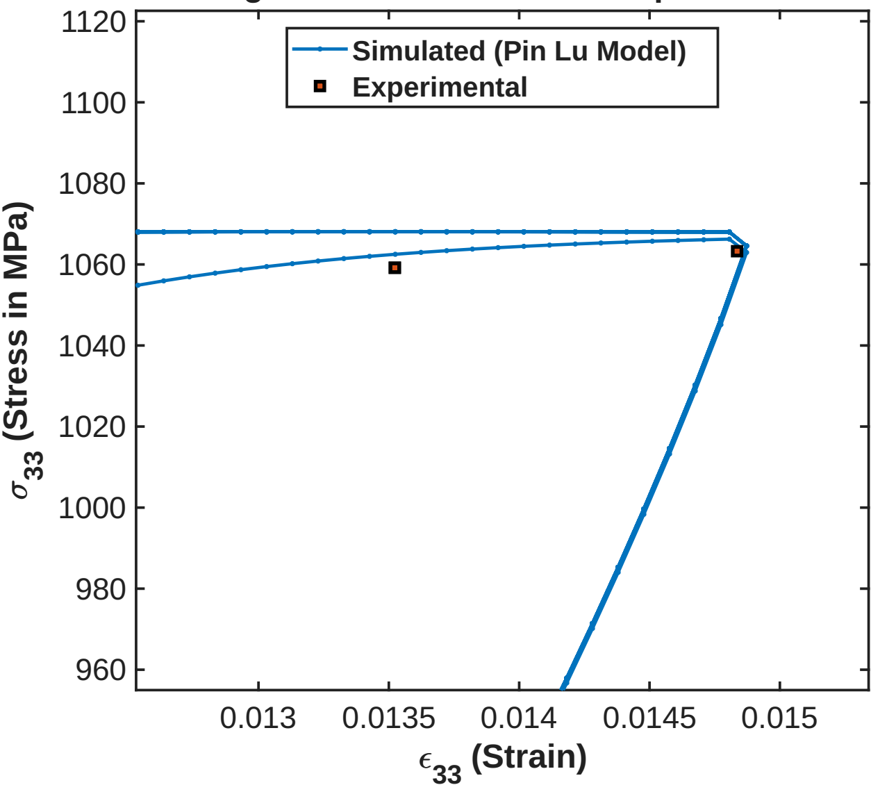
Fatigue Test: Simulated vs Experimental
